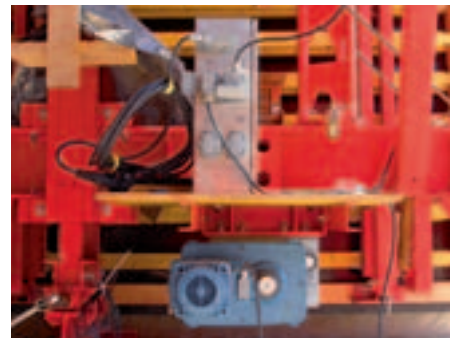
If required, the electric drive can be used for moving purposes. It can be retro-fitted on the wheel.
