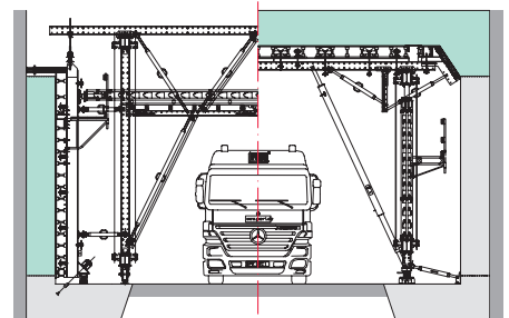
Clearly visible are the 2 separate concreting cycles, the wall on the left and the slab on the right. Both sets of formworks are designed as mobile units.
