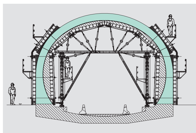
Circular cross-sections are also just as possible as separate individual formwork carriages for walls and slabs.
