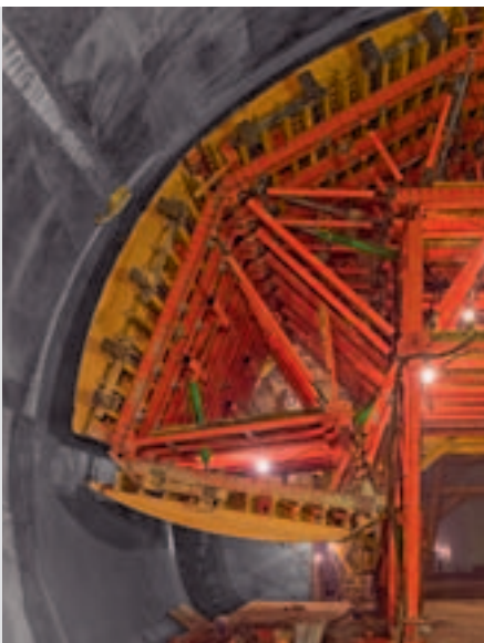
Optional VARIOKIT accessories such as hydraulic winches, electric drive units, lifting and lowering units and hydraulic cylinders for operating the wall and slab formwork elements are available in the VARIOKIT construction kit and, if necessary, are planned according to project requirements.
