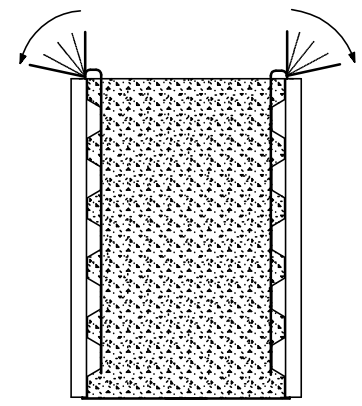
Close formwork with S-hook fix by bending the round steel bar ends. Place concrete
