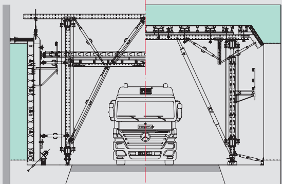
Clearly visible are the 2 separate concreting cycles, the wall on the left and the slab on the right. Both sets of formwork are designed as mobile units.
