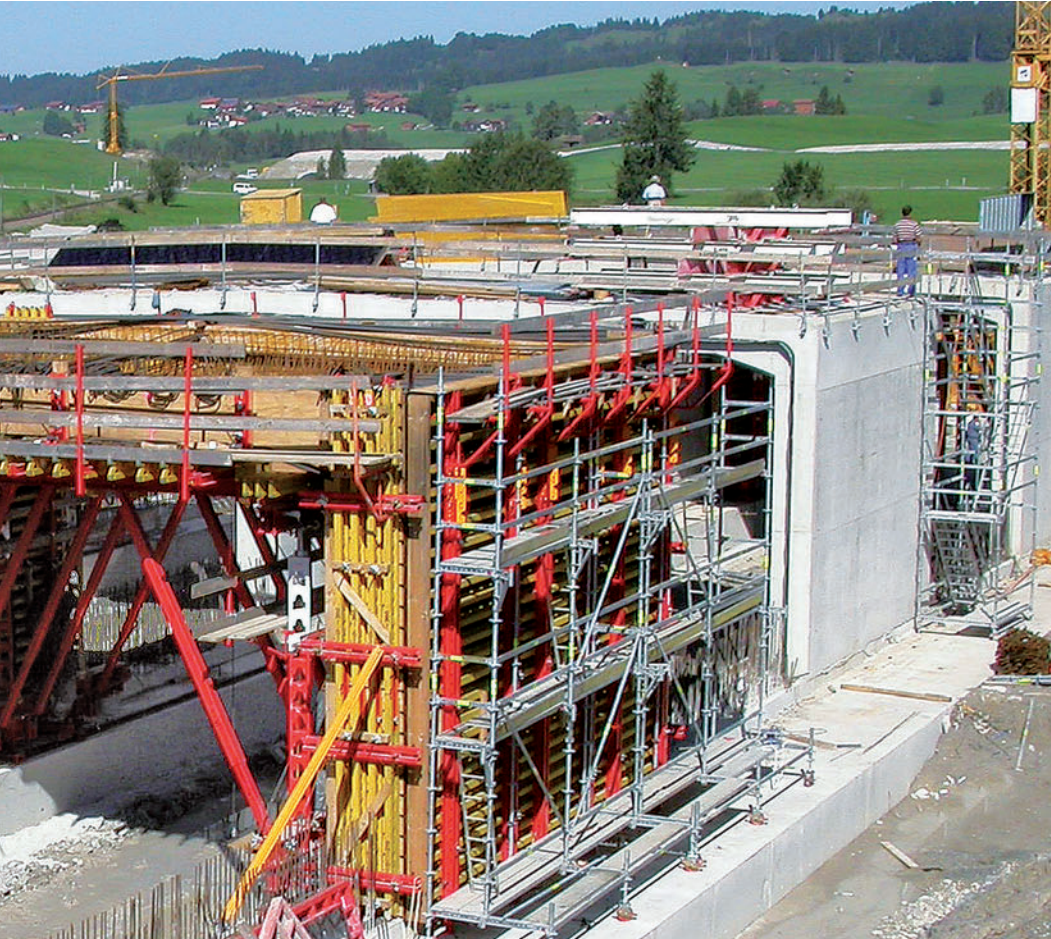
The combination of proven systems such as VARIO GT 24 and HD 200 with new elements from RCS or the diagonal strut, results in a cost-effective formwork carriage.
