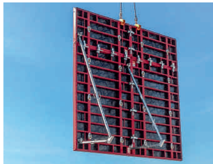
... moving the preassembled wall formwork units including push-pull props with the crane ...
